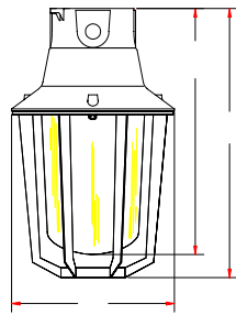
CEILING MOUNT
